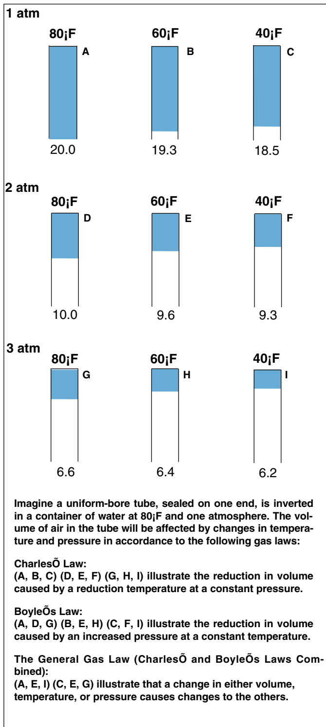
FIGURE 2.8 Gas Laws
